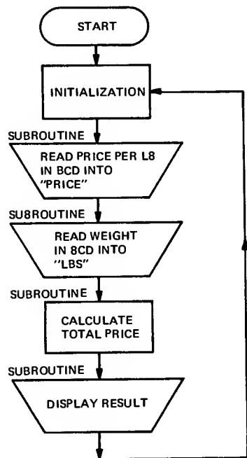
Fig. 120 – Over-all program flow chart for microcomputer scale.
