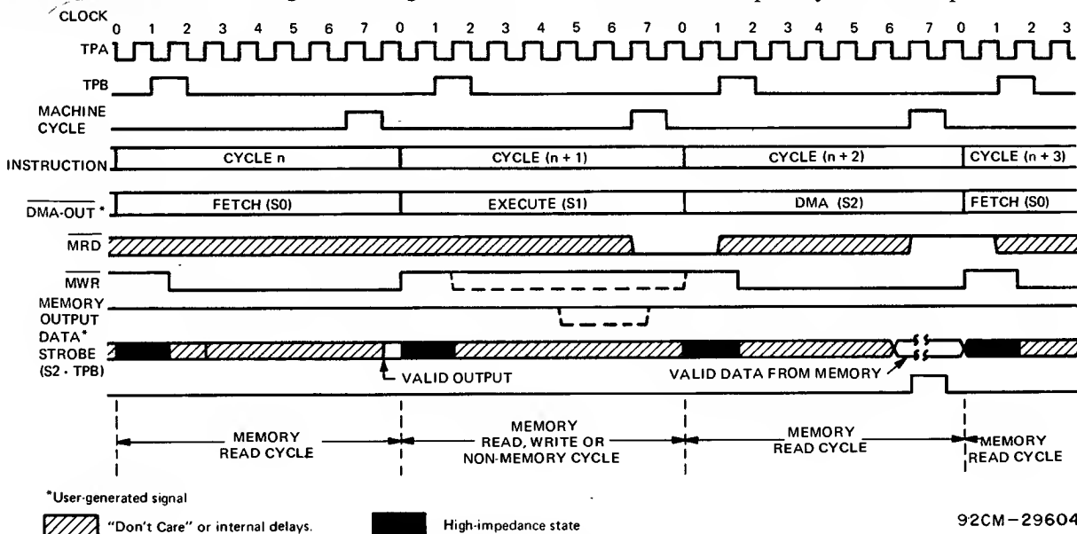
Fig. 114 - DMA-OUT timing.
