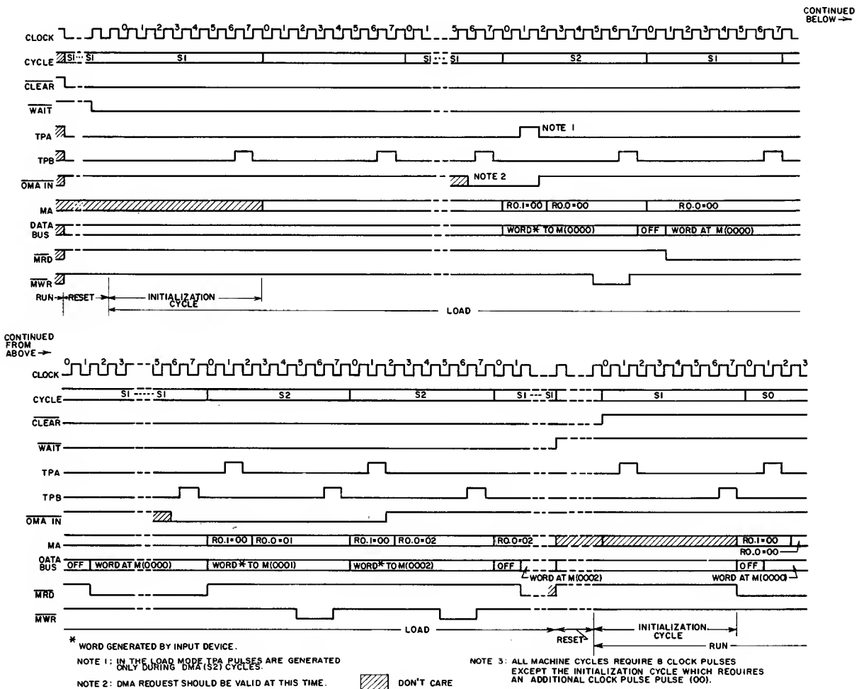
Fig. 85 - Timing diagram for run and load sequences.
