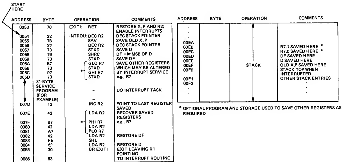
Fig. 76 - Interrupt service routine.
